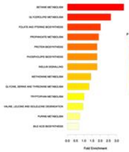
A Metabolite Sets Enrichment Overview
