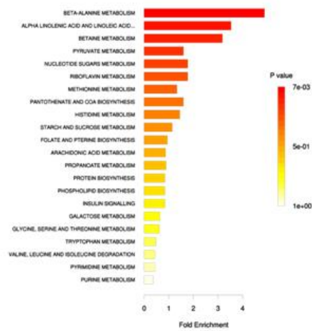
A Metabolite Sets Enrichment Overview
